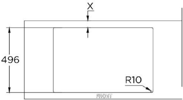
INSTALLATION STANDARD
